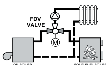
Changeover application
