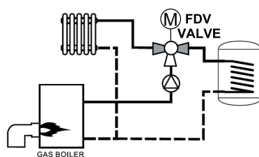
Diverting application
